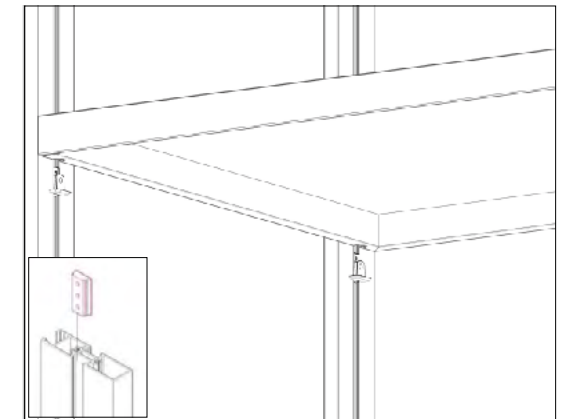
Raf Braketleri Shelf Bracket
