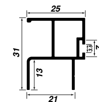
18 mm Aluminium Side Handle
