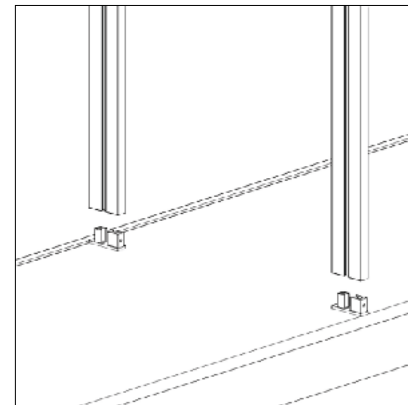
Alüminyum I Profil Alt Panel Montaj Aluminium I Profile Bottom and Top Panel Mounting
