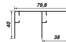
Aluminium 34mm Upper Double Rail
