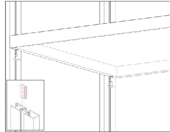
Raf Braket Shelf Bracket
